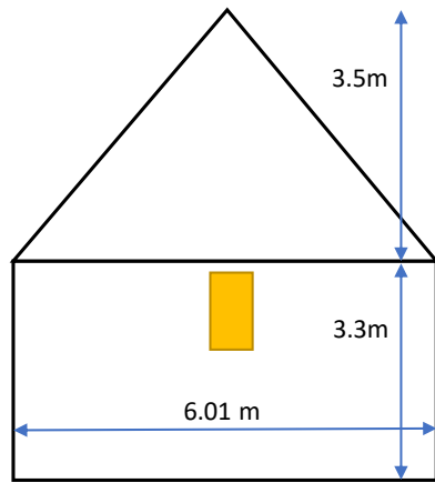
end elevation (North)
